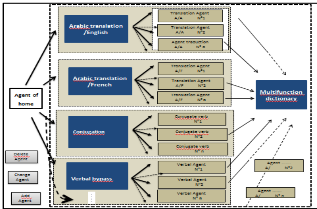
Fig. 3. General architecture of the multi-agents system "Feedback"
