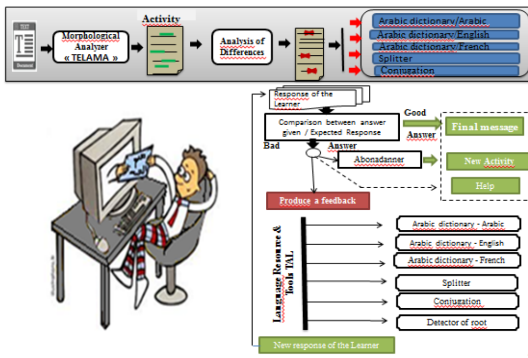
Fig. 2. Feedback: Integration of language resources in TELA
